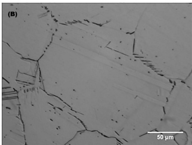
Figure A.18—Unacceptable Microstructure for UNS N07716, UNS N07725, UNS N09925, UNS N09935, UNS N09945, UNS N09946 and UNS N09955 Showing Acicular Grain Boundary Precipitates; Original Magnification: 100X for Upper Photomicrograph (A); 500X for Lower Photomicrograph (B)
