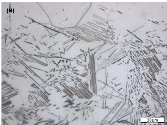
Figure A.19—Unacceptable Microstructure for UNS N07716, UNS N07725, UNS N09925, UNS N09935, UNS N09945, UNS N09946 and UNS N09955 Due to Acicular Precipitates; Original Magnification: 100X for Upper Photomicrograph (A); 500X for Lower Photomicrograph (B)
