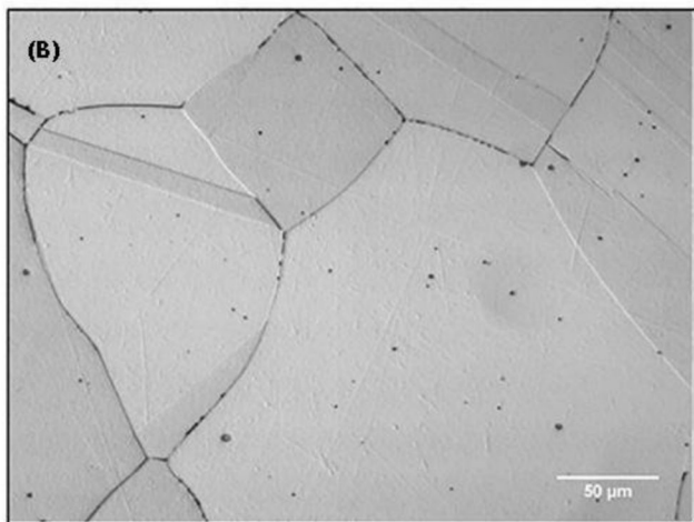
Figure A.16—Acceptable Microstructure for UNS N07716, UNS N07725, UNS N09925, UNS N09935, UNS N09945, UNS N09946 and UNS N09955 Showing Partial Coverage of Grain Boundaries with Second Phase Particles; Original Magnification: 100X for Upper Photomicrograph (A); 500X for Lower Photomicrograph (B)
