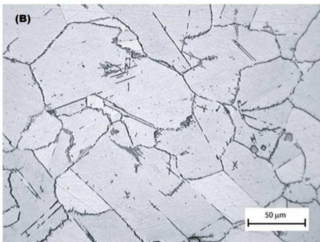
Figure A.6—Unacceptable Microstructure for UNS N07718 Showing Acicular Grain Boundary Precipitates; Original Magnification: 100X for Upper Photomicrograph (A); 500X for Lower Photomicrograph (B)
