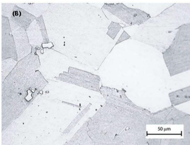
Figure A.1—Acceptable Microstructure for UNS N07718; Original Magnification: 100X for Upper Photomicrograph (A); 500X for Lower Photomicrograph (B)
