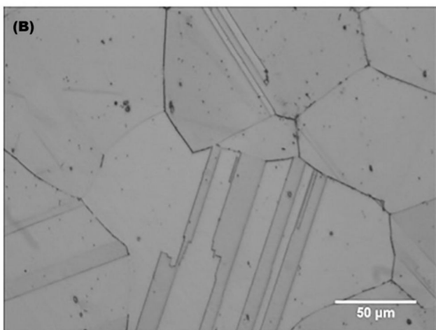
Figure A.15—Acceptable Microstructure for UNS N07716, UNS N07725, UNS N09925, UNS N09935, UNS N09945, UNS N09946 and UNS N09955 Showing Partial Coverage of Grain Boundaries with Second Phase Particles; Original Magnification: 100X for Upper Photomicrograph (A); 500X for Lower Photomicrograph (B)
