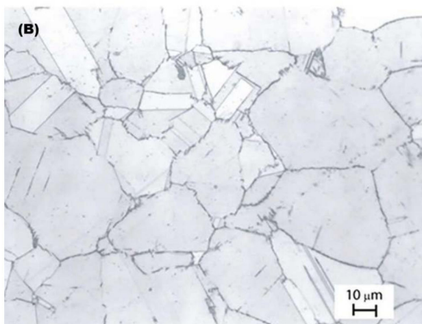
Figure A.5—Unacceptable Microstructure for UNS N07718 Showing Acicular Grain Boundary Precipitates; Original Magnification: 100X for Upper Photomicrograph (A); 500X for Lower Photomicrograph (B)
