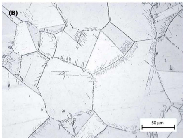
Figure A.7—Unacceptable Microstructure for UNS N07718 Showing Acicular Grain Boundary Precipitates; Original Magnification: 100X for Upper Photomicrograph (A); 500X for Lower Photomicrograph (B)
