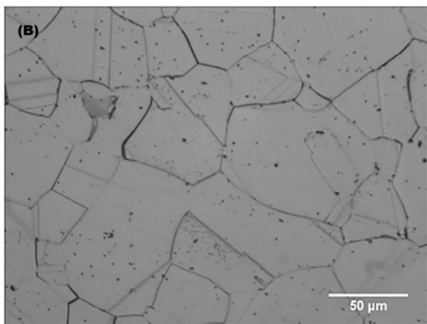
Figure A.14—Acceptable Microstructure for UNS N07716, UNS N07725, UNS N09925, UNS N09935, UNS N09945, UNS N09946 and UNS N09955 Showing Isolated Grain Boundary Precipitation; Original Magnification: 100X for Upper Photomicrograph (A); 500X for Lower Photomicrograph (B)
