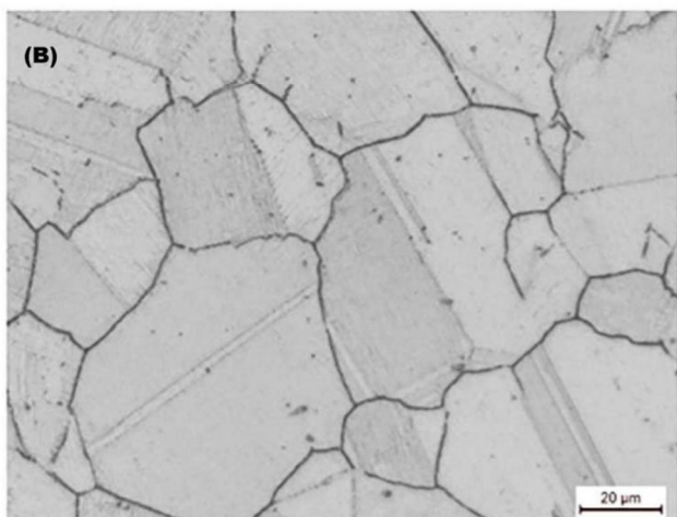
Figure A.17—Unacceptable Microstructure for UNS N07716, UNS N07725, UNS N09925, UNS N09935, UNS N09945, UNS N09946 and UNS N09955 Showing Full Coverage of Grain Boundaries with Second Phase Particles; Original Magnification: 100X for Upper Photomicrograph (A); 500X for Lower Photomicrograph (B)
