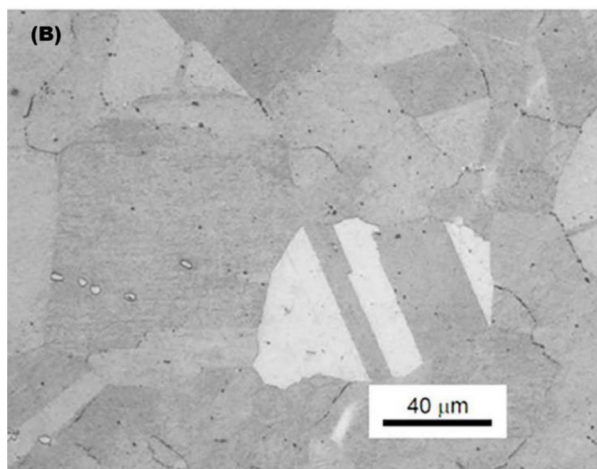
Figure A.4—Acceptable Microstructure for UNS N07718 Showing Isolated Acicular Grain Boundary Precipitates; Original Magnification: 100X for Upper Photomicrograph (A); 500X for Lower Photomicrograph (B)
