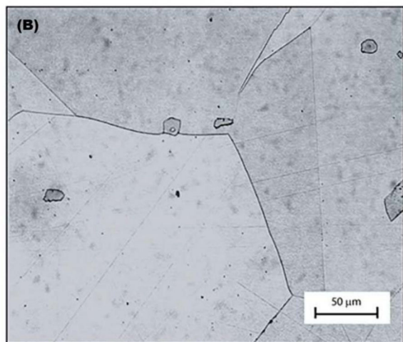
Figure A.3—Acceptable Microstructure for UNS N07718 Showing Isolated Grain Boundary Precipitates; Original Magnification: 100X for Upper Photomicrograph (A); 500X for Lower Photomicrograph (B)
