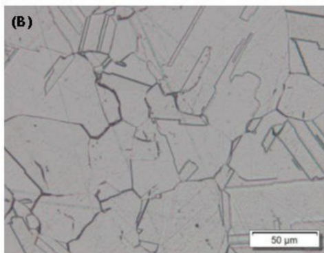
Figure A.11—Acceptable Microstructure for UNS N06625; Original Magnification: 100X for Upper Photomicrograph (A); 500X for Lower Photomicrograph (B)
