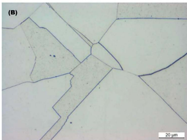
Figure A.13—Acceptable Microstructure for UNS N07716, UNS N07725, UNS N09925, UNS N09935, UNS N09945, UNS N09946 and UNS N09955; Original Magnification: 100X for Upper Photomicrograph (A); 500X for Lower Photomicrograph (B)
